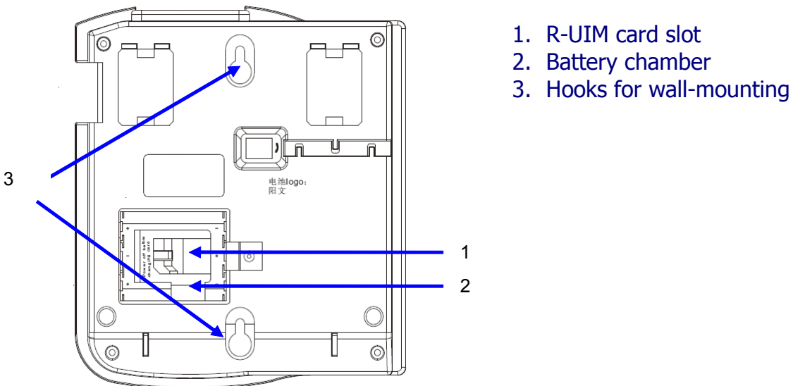
Figure 2 Backside of the Phone
